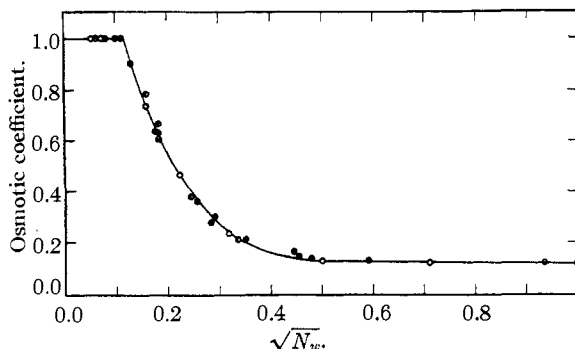
Fig. 4.—Osmotic coefficients of dodecylamine salts in water: \otimes formate, \circ acetate, \bullet propionate, \ominus N-dimethylammonium chloride, \ominus N-dimethylammonium acetate.
