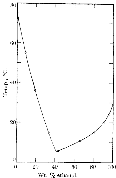
Fig. 7.—Solution temperatures of 50.0% dodecylammonium acetate in aqueous ethanol.
